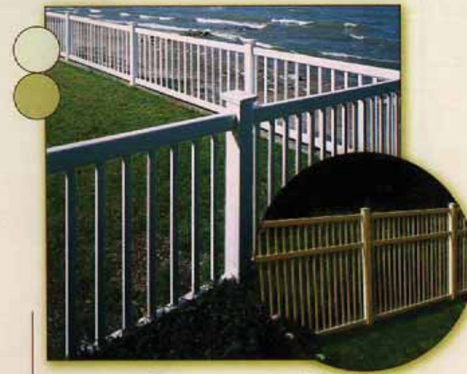
VICTORIAN/VICTORIAN WITH MIDRAIL Heights: 3', 4', 5' & 6' (5' & 6' include midrail) Colors: White & Tan Picket Style: 7/8" x 1-1/2"
